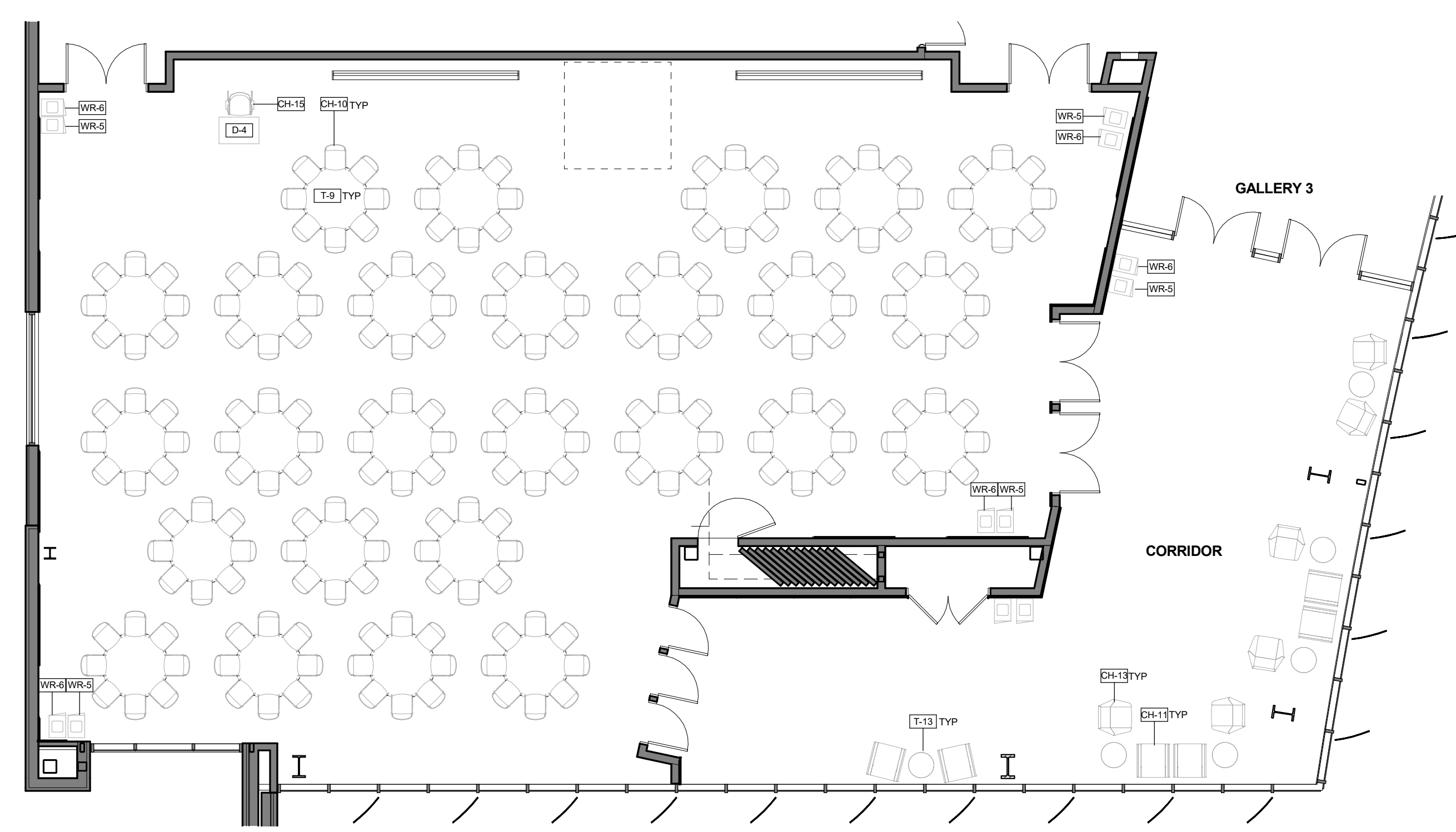
A1 3RD FLOOR BANQUET SET UP 1/8" = 1'-0"
